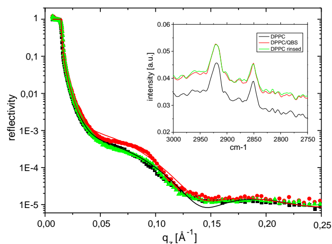
Fig. 9. Neutron reflectivity curves and FTIR ATR spectra (inset) at the Si/water interface (20 °C) of DPPC bilayers in pure D_2O (black squares), DPPC bilayers penetrated with QBS (red circles) and of the same system after exchange of QBS back with D_2O (green triangles). The values of the fit (straight line) are given in the text.
